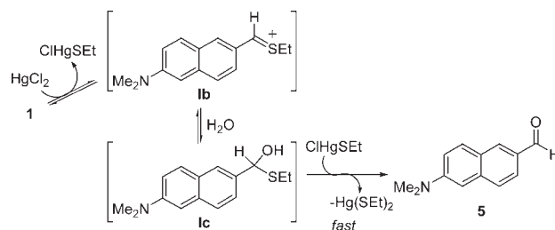
Scheme 3. Mechanism of \text{Hg}^{2+} -Promoted Conversion of DTA 1 to Aldehyde 5 with 1 equiv of \text{HgCl}_2
